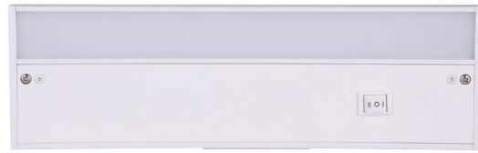
CUC1012-W-LED - 12" Light Bar 6 Watt LED; 370 Lumens, 3000k, 90 CRI, Dimmable 12"L x 3.63"W x 1"H; Frosted Polycarbonate Lens Finishes: BZ, W
